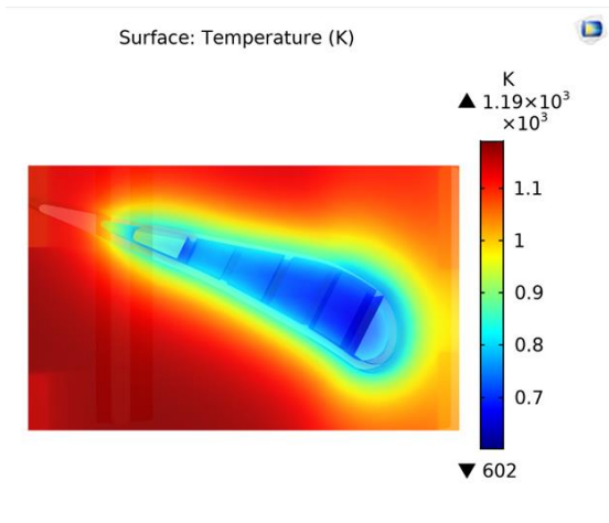
Figure 10. The temperature distribution in case of Helium coolant
