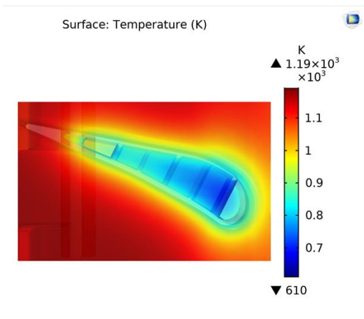
Figure 12. The temperature distribution in case of steam coolant
