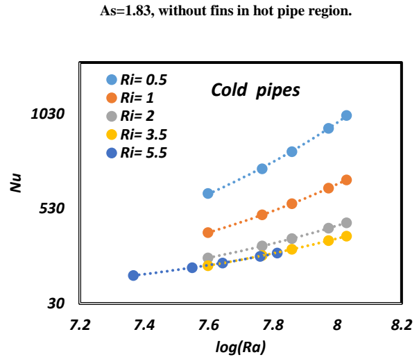
Figure 4. Nusselt number vs. Rayleigh number for various Ri , As=1.83 , without fins in cold pipe region.
