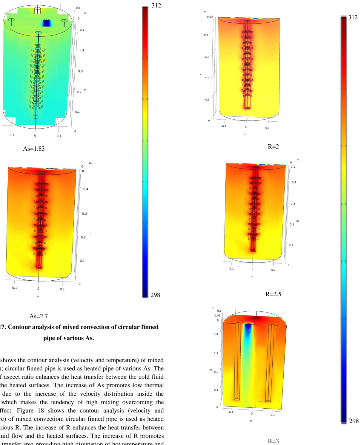
Figure 18. Contour analysis of mixed convection of circular finned pipe of various R .
